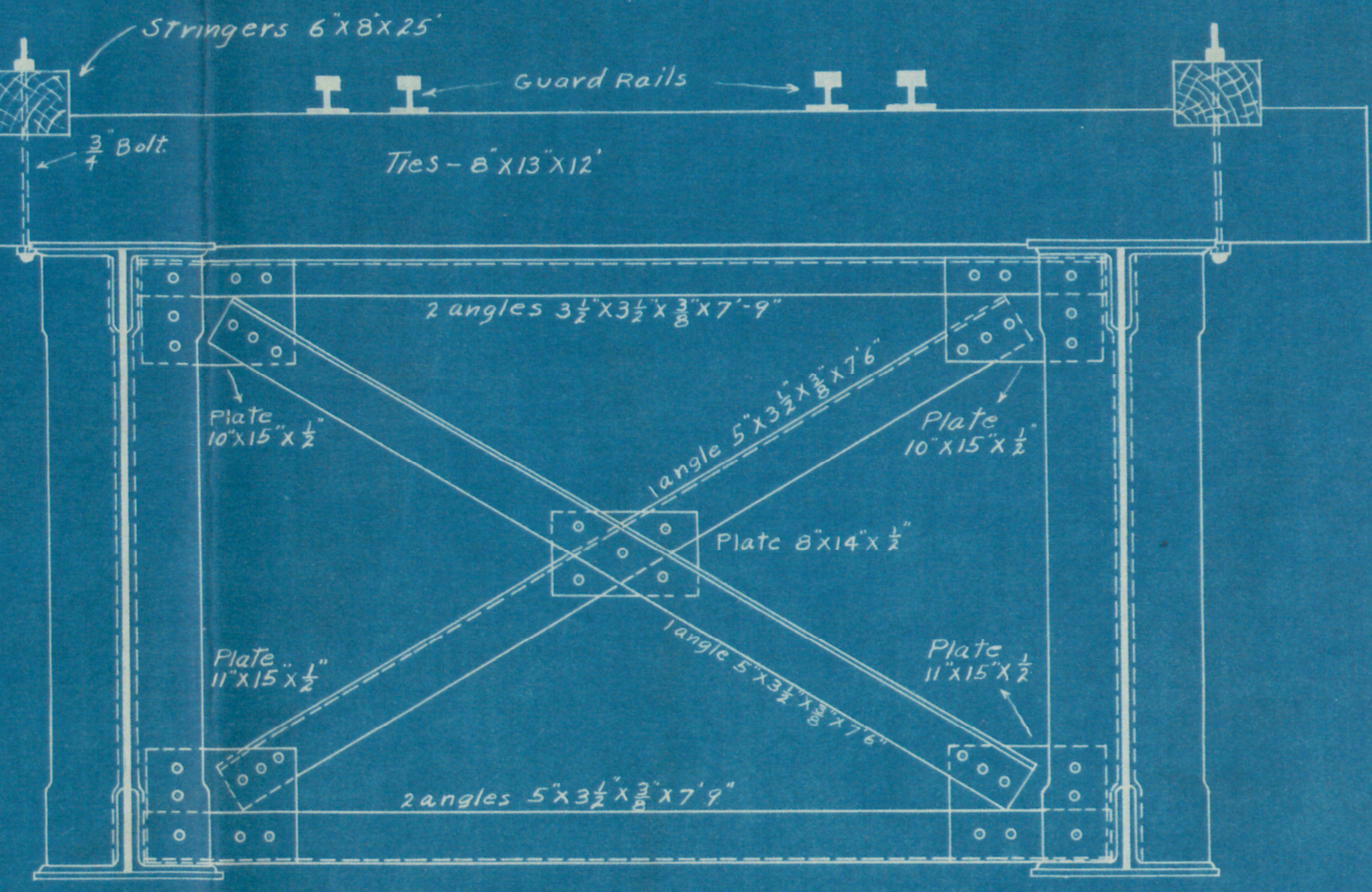
End Cross Frame.
