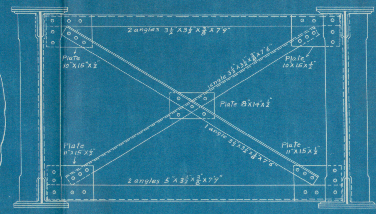
Intermediate Cross Frame.
