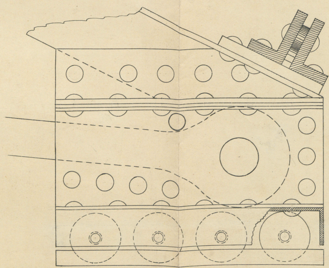
Side View of Shoe-Plate One-Fourth Size
